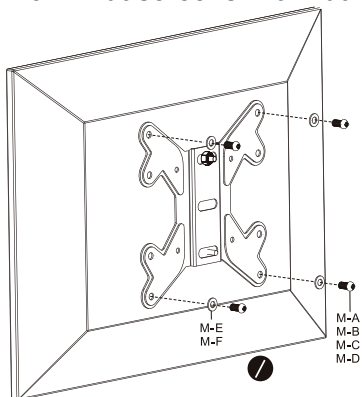
Fig. 18: Flat screens with flat back
