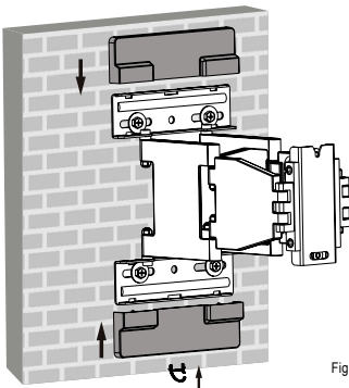
Fig. 4: Wandmontage
