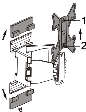
Fig. 12: Removing plastic covers and VESA plate
