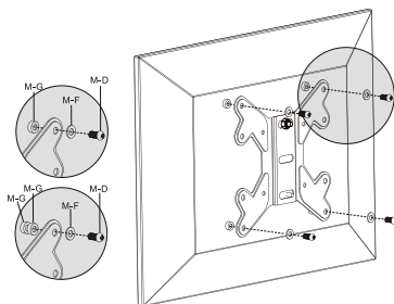
Fig. 19: Flat screens with arched back
