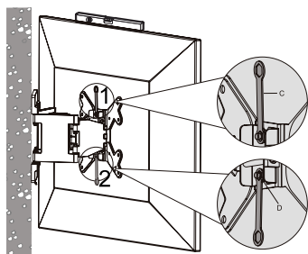
Fig. 21: Fixing the flat screen
