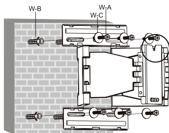
Fig. 15: Wall mounting
