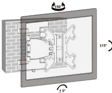
Fig. 22: Aligning the flat screen
