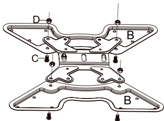
Fig. 17: Mounting the flat screen
